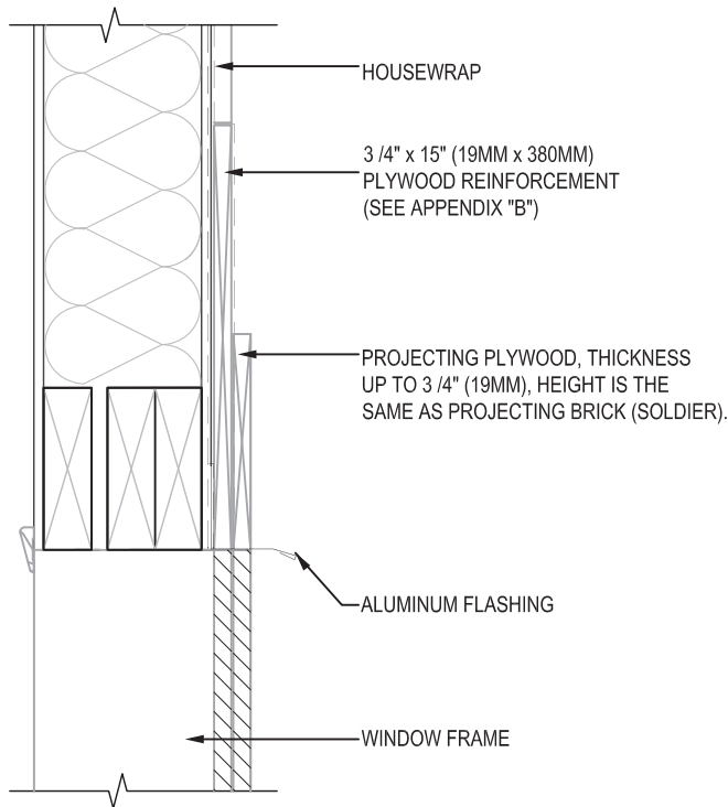
WINDOW HEADER SECTION
