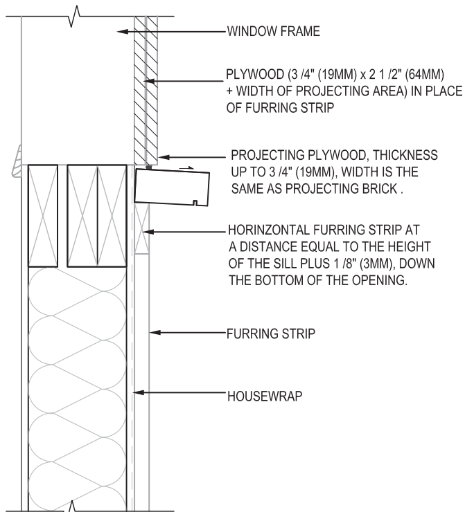
WINDOW SILL SECTION
