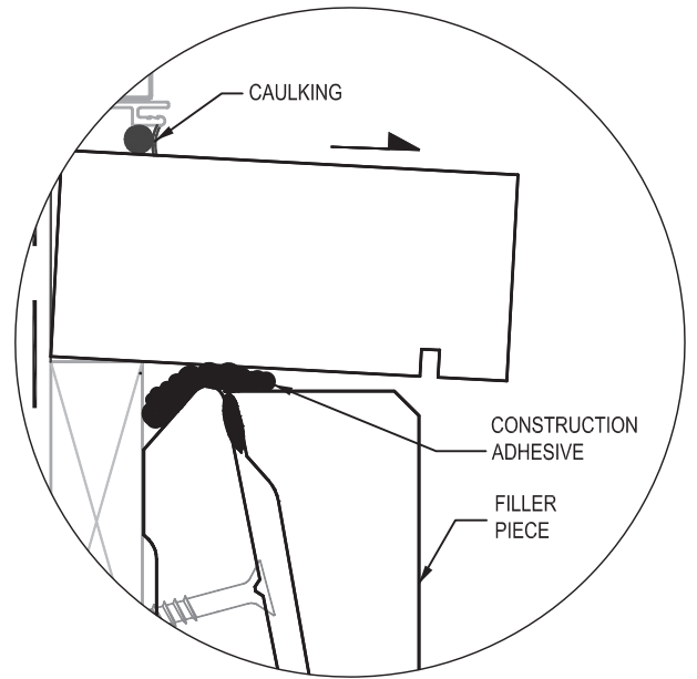
Sill detail
